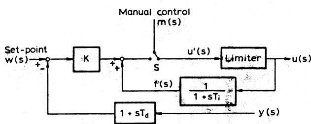
Fig 4 Practical PID block diagram
