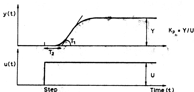
Fig 10 Open-loop step test on a process
