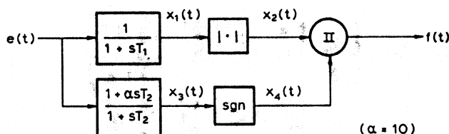
Fig 8 A non-linear phase-lead filter
